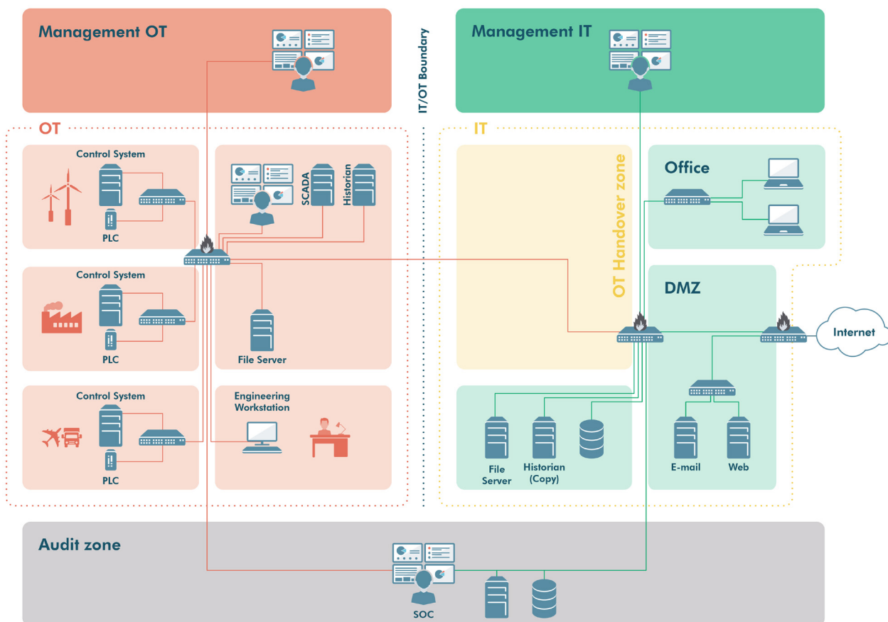
Figure 1. Zones in IT/OT environment without high assurance solutions
