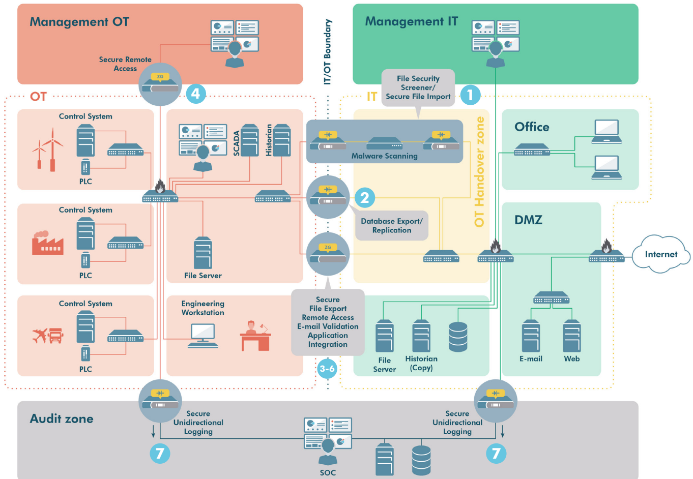
Figure 2. Zones in IT/OT environment with high assurance solutions
