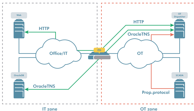
ZoneGuard with HTTP and OracleTNS protocol validation services, validates traffic flow between the OT Dispatcher and the systems located in the IT zone
